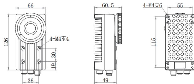
MV-SI622-30GM
