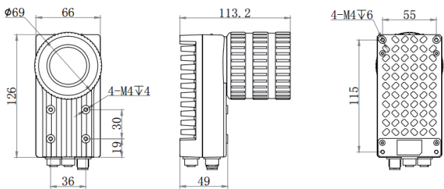
MV-SI622-31GM
